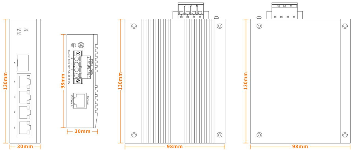
SFP model
