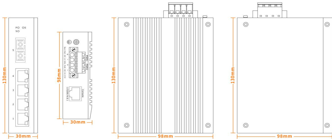
SC/FC/ST model
